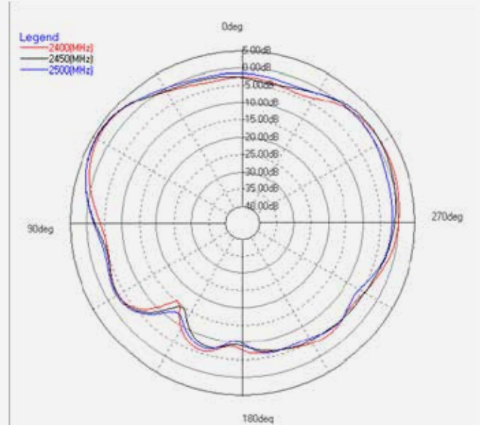
2.4G (PHI=90)
