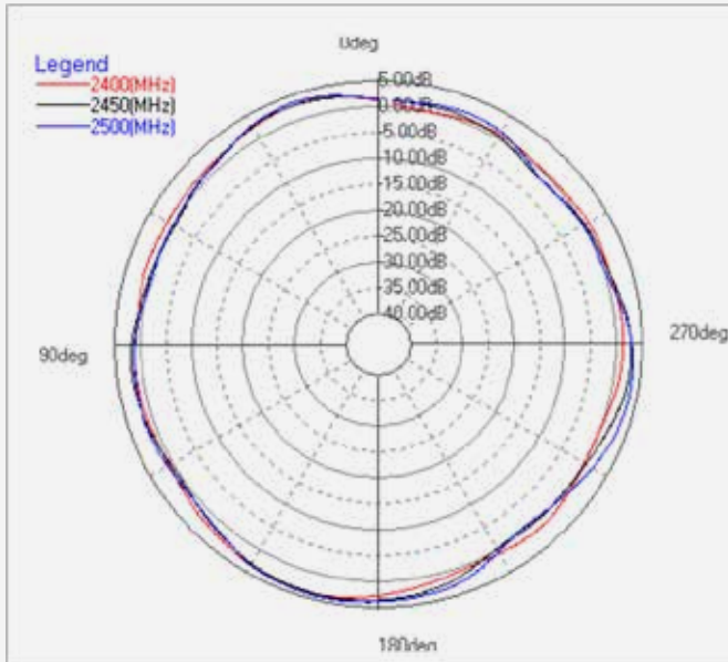
2.4G (PHI=0)
